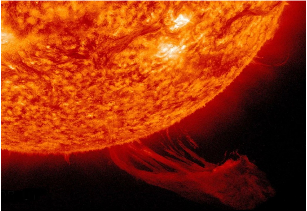
A solar prominence rose up and swept away from the sun as captured in this image at 4:15 a.m. EDT on Oct. 19, 2012. https://www.nbcnews.com/id/wbna49483655
