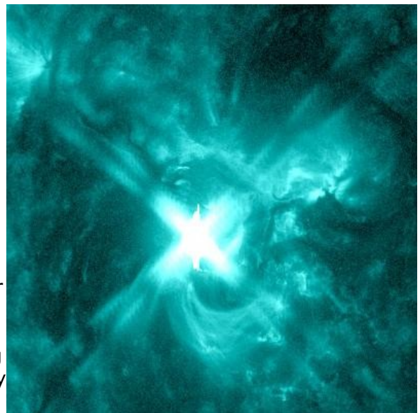
X CLASS SOLAR FLARE in last 2 days
